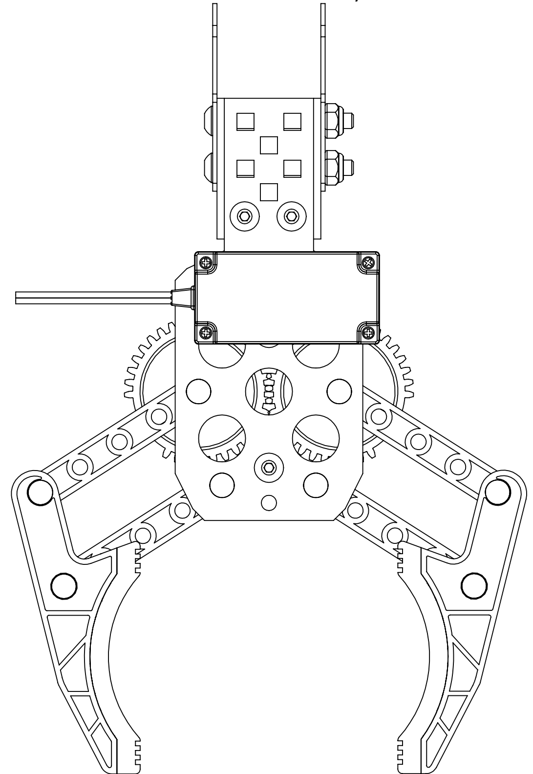
Claw Assembly
