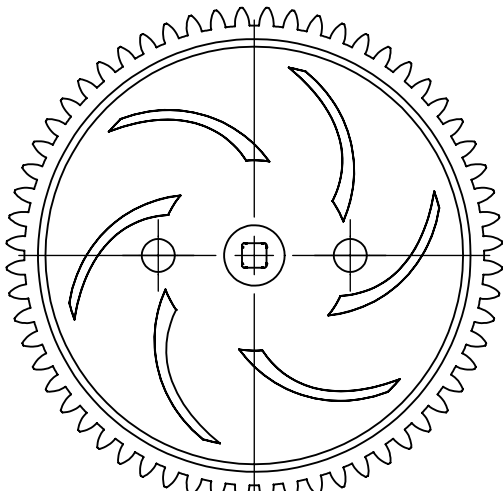
60-TOOTH GEAR (2)
