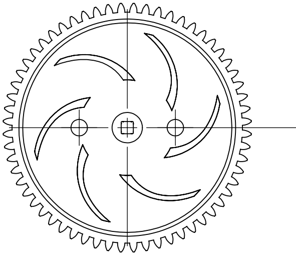
60-TOOTH GEAR (2)
